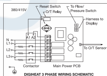
DigiHeat 3 Phase
